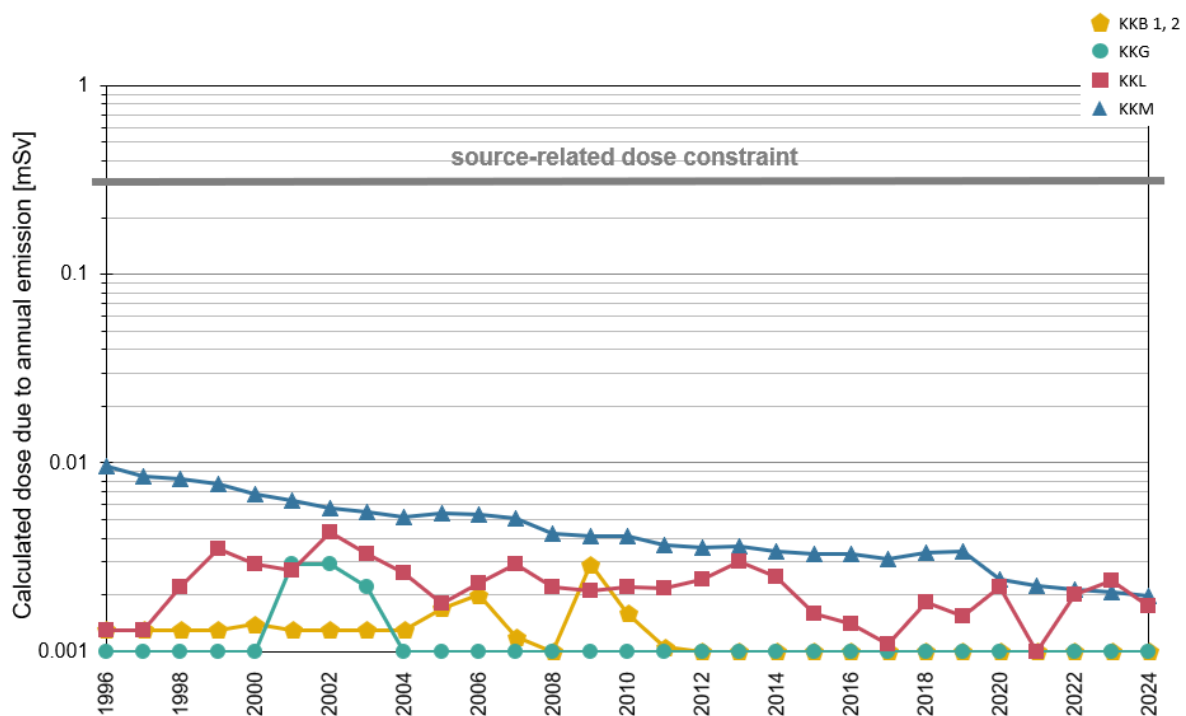
Figure 7: Doses calculated based on annual emissions from the Swiss NPPs without the contribution of direct radiation. The annual doses are calculated for a virtual most exposed group of the population, including the exposure due to deposition from former years. The source-related dose constraint of 0.3 mSv/year is also shown. (note 1: the Beznau NPP consists of two units, both located on the same site; note 2: the Mühleberg NPP has permanently ceased operation and is in decommissioning since 2020)
