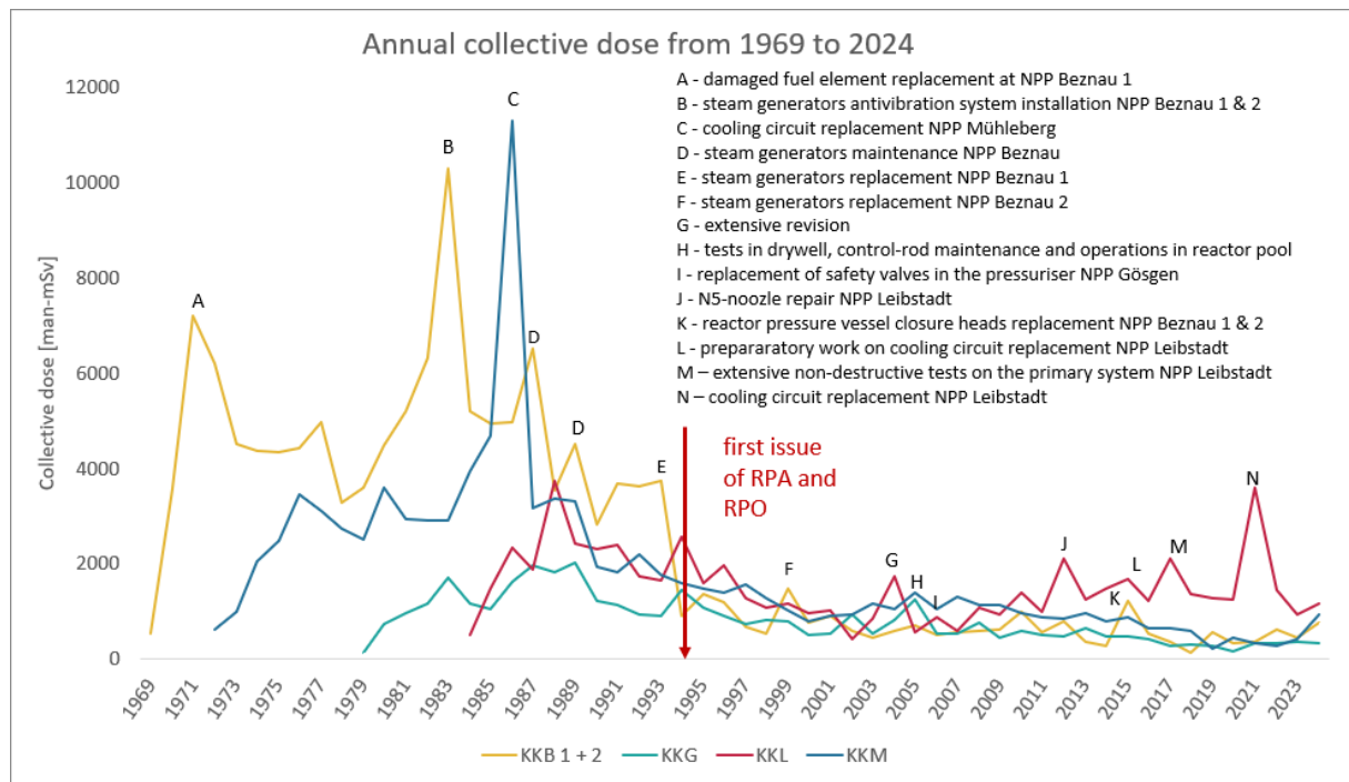
Figure 6: Annual collective doses for the personnel in Swiss NPPs. All peaks relate to extraordinary work performed. (note 1: the Beznau NPP consists of two units, both located on the same site; note 2: the Mühleberg NPP has permanently ceased operation and is in decommissioning since 2020).
